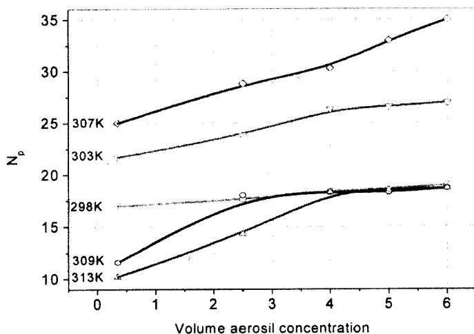
FIGURE 5 Number of aerosil particles in the aggregate vs aerosil concentration in the suspension.
