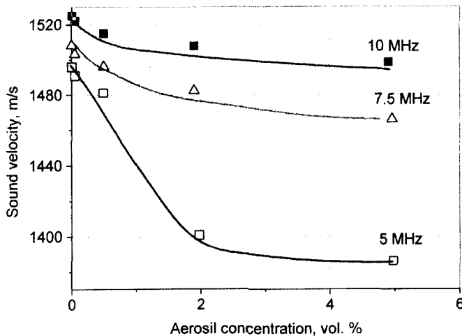
FIGURE 2 Dependence of the sound velocity on the volume fraction of aerosil in the suspension.
