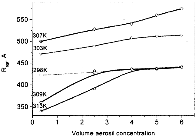
FIGURE 4 Aerosil aggregate size vs aerosil concentration.
