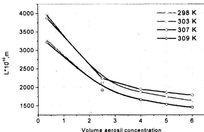
FIGURE 7 Distance between the aggregates vs aerosil concentration.
