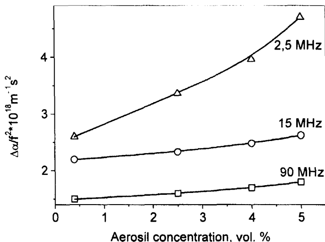
FIGURE 3 The redundant sound absorption vs aerosil concentration.
